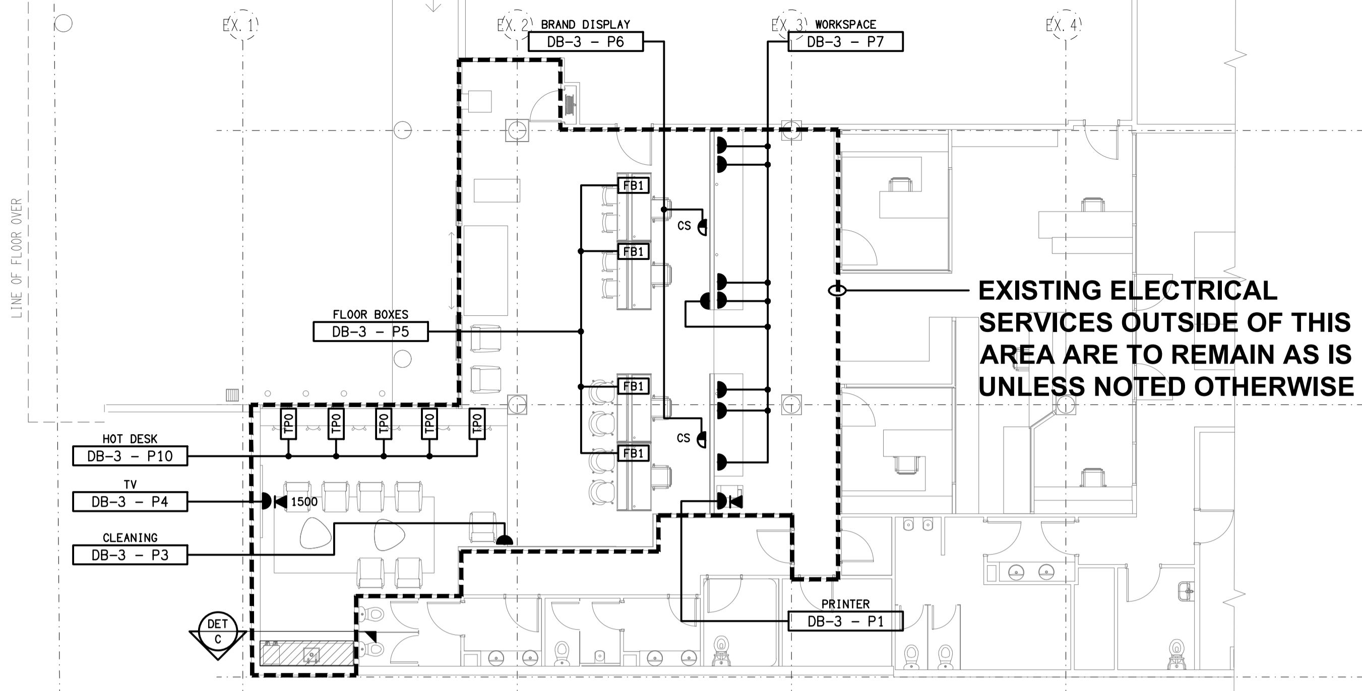
LOWER LEVEL FLOOR PLAN SCALE 1:100
